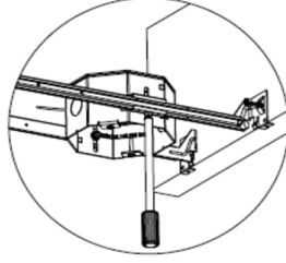
3. Slide junction box to desired location along and then fix into place along channels with screws
