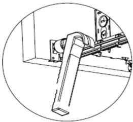
2. Attach hanger bars to wooden joist
