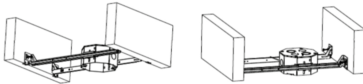
1. Position hanger bar/junction box assembly on wooden joist as shown
