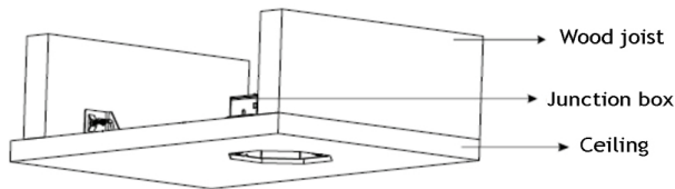
3. Slide junction box to desired location along and then fix into place along channels with screws
