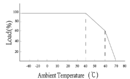
Load vs Ambient Temp Curve
