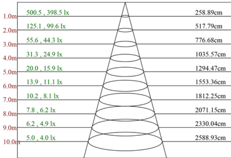
Max , Ave Beam angle of C0plane 104.62
