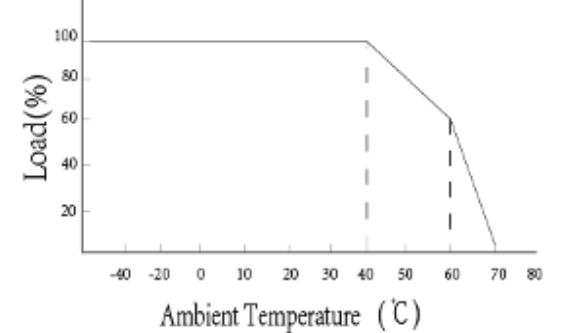
Load vs Ambient Temp Curve
