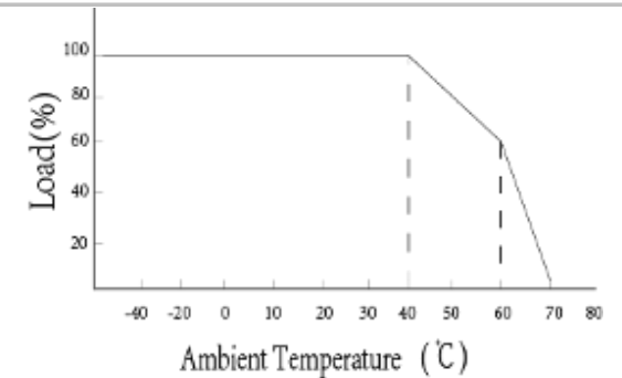
Load vs Ambient Temp Curve
