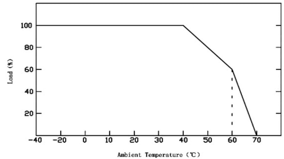
Derating Curve - Load according to this diagram
